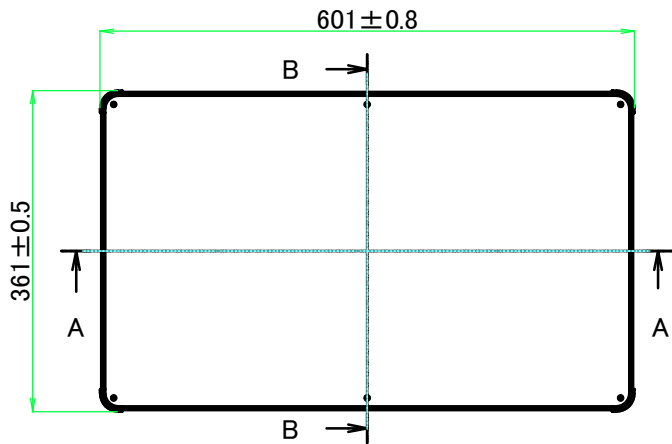
E view
